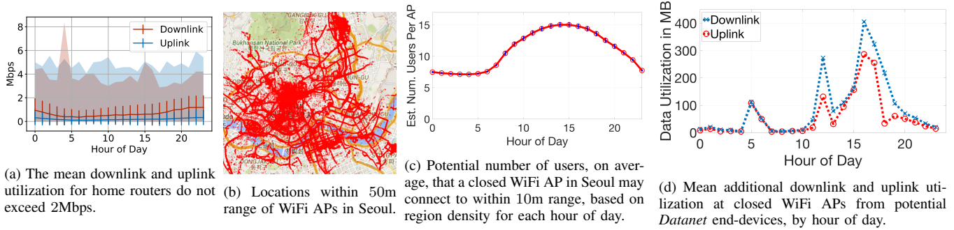
Fig. 2: Depicting (a) underutilization of typical home routers, and (b,c, d) potential benefit to private APs in Seoul by serving data needs of devices accessible through Datanet .
